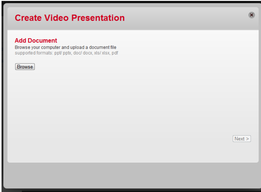
Figure 7: Select Document
